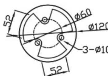
PLATE DETAIL
